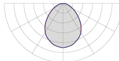
Photometric curve
